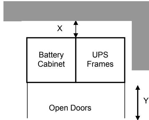
Figure 2 : : UPS + Battery space recommendation
