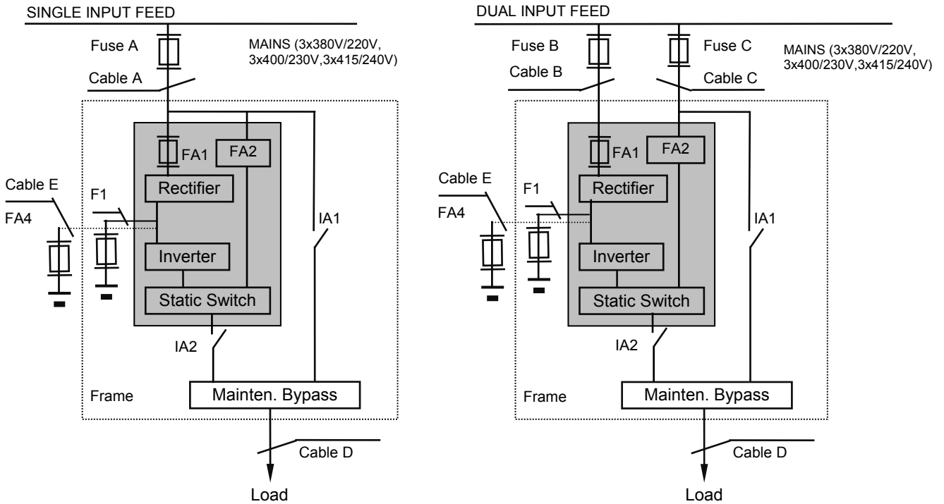
Figure 3.3: Block Diagram POWERSCALE from 10-50 kVA
